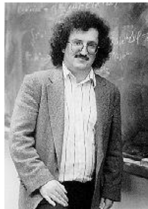
Fig. 3. Professor Paweł Oskar Mazur before 1982, picture is taken from his homepage in USC.
